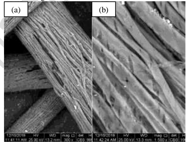
Figure 2. SEM micrographs of date palm petioles: (a) 300 \mu m , (b) 50 \mu m .
