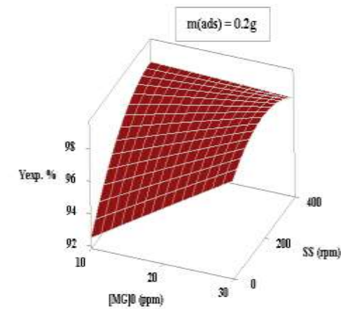
Figure 9. Response surface of yield according to [MG]_0 and SS (at m_{ads} = 0.2g ).
