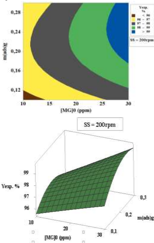
Figure 7. Response surface of yield according to [MG] 0 and m ads (at m ads = 200rpm).
