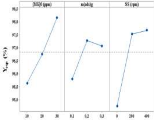
Figure 5. Main effects plot of parameters for yield.
