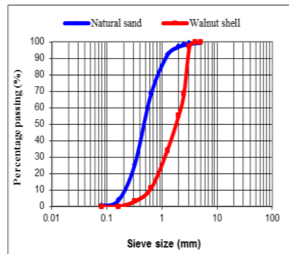
Figure 2. Particle size distribution of natural sand and walnut shell waste.
