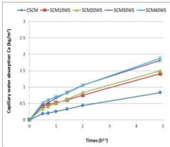
Figure 10. Effect of walnut shell content on capillary water absorption of SCM mixes.
