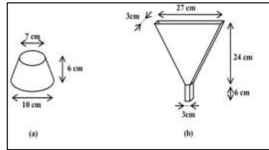
Figure 3. Workability tests for fresh SCM mixes (a/ Mini-slump flow test; b/ V-funnel test)..
