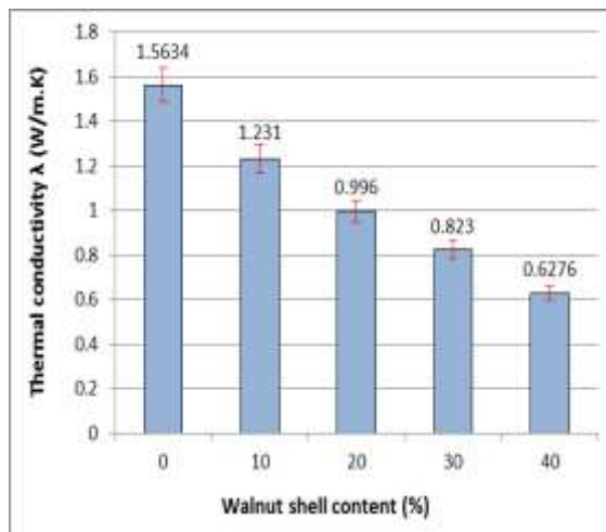
Figure 8. Effect of walnut shell content on thermal conductivity of SCM mixes.
