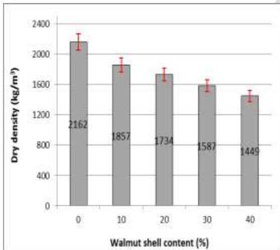
Figure 6. Effect of walnut shell content on dry density of SCM mixes.
