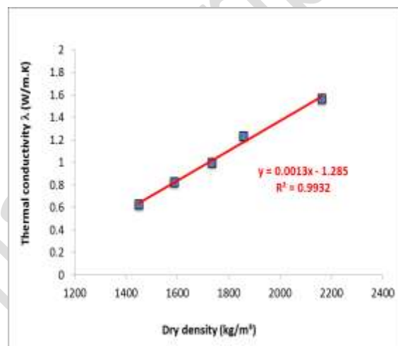
Figure 9. Relation between thermal conductivity and dry density of SCM containing walnut shell.
