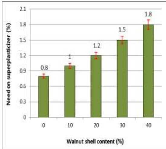
Figure 5. Effect of walnut shell content on the need on superplasticizer of SCM mixes.
