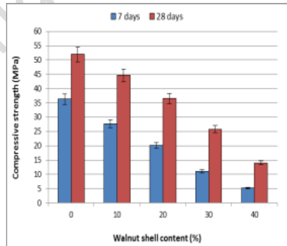
Figure 7. Effect of walnut shell content on compressive strength of SCM mixes.
