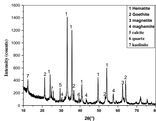
Figure 3. DRX spectrum of Gara-Djebilet iron ores.
